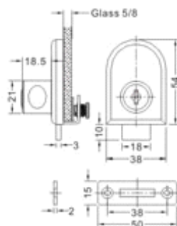
ABD-707 Cabinet Glass Door Lock(For Single Doors)
