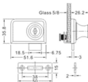
ABD-709 Cabinet Glass Door Lock(For Double Doors)
