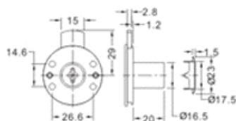
ABD-703 Cupboard Lock
