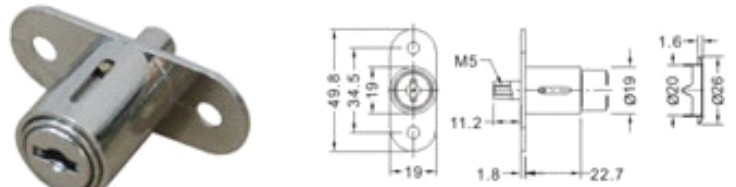
ABD-714 Push Lock
