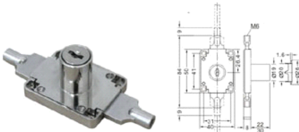
ABD-713 Extending Bar Lock
