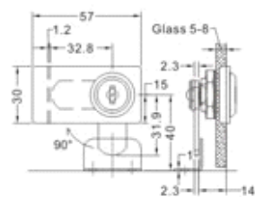
ABD-710 Cabinet Glass Door Lock(For Double Doors)
