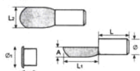
Metal Shelf Support
