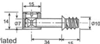
Strong Fittings 4 in 1 (6mm)
