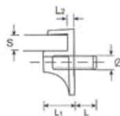
Plastic Board Support
