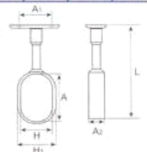
Hanging Rail Tube Support
