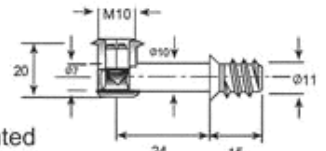
Strong Fittings 4 in 1 (8mm)
