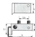
Cabinet Suspension Bracket
