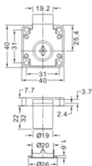
ABD-701 Drawer Lock
