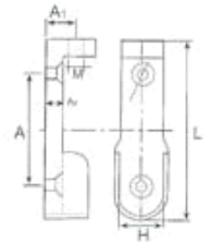
Hanging Rail Tube Support
