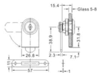
ABD-708 Cabinet Glass Door Lock(For Single Doors)
