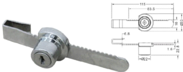
ABD-711 Push-Type Glass Door Lock
