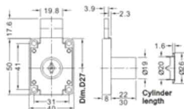
ABD-702 Two Turns & Long Latch Lock
